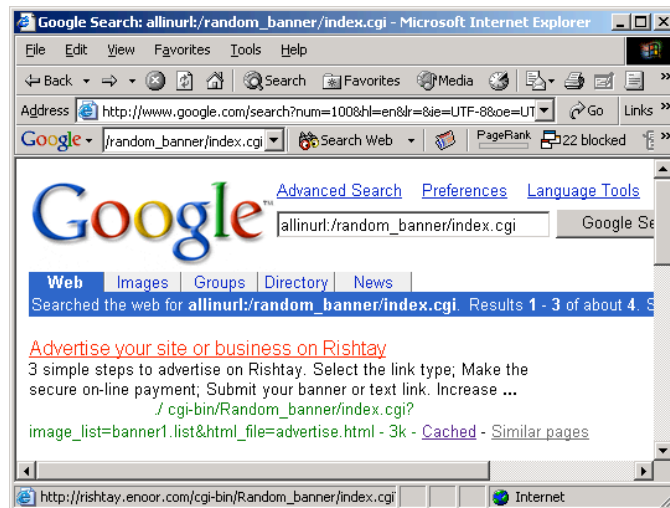
Figure 15: Example search using a line from a CGI scanner
